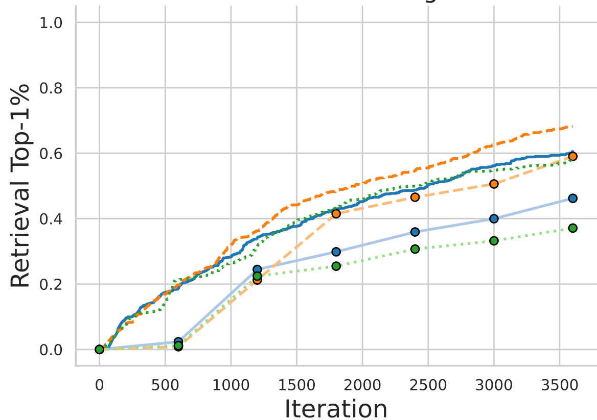
Score = Docking
