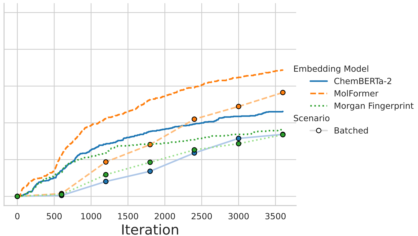
Score = MMGBSA
